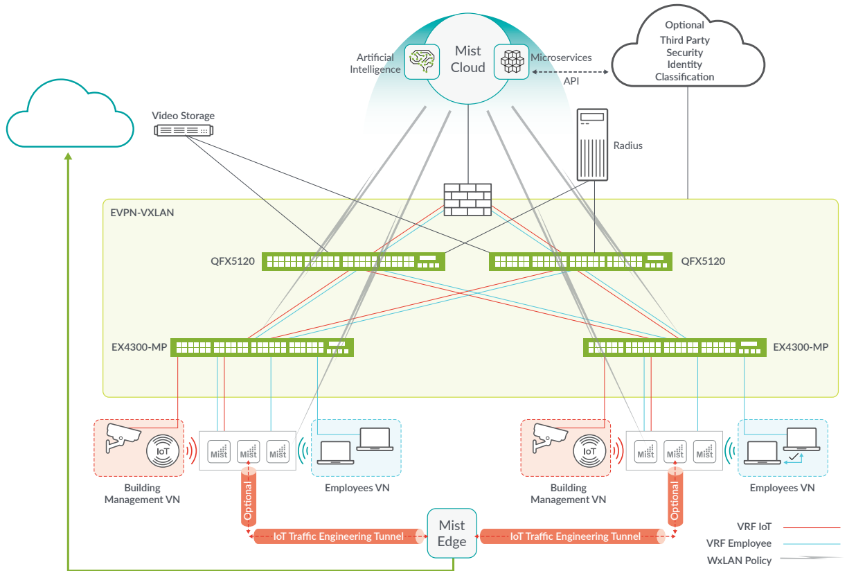
Figure 7: Network segmentation based on employee or device profile
