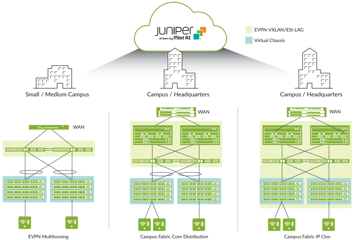
Figure 2: Campus fabrics showing Virtual Chassis and EVPN-VXLAN based architectures.
